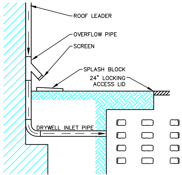
OVERFLOW DETAIL
